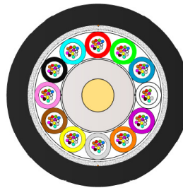
12 Elements Cable
